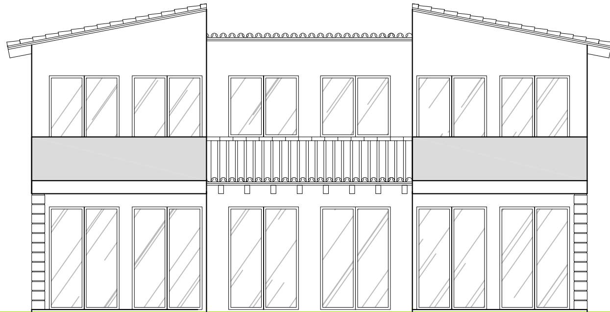
ALZADO PRINCIPAL
